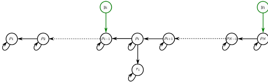
Fig. 2. The graph \mathcal{G}(\mathcal{A}^T, \mathcal{C}^T) for patterns \mathcal{A} and \mathcal{C} that include matrices A and C , respectively, of system (10), (11), for the case of a simple one-lane highway stretch with N segments (Model I).
