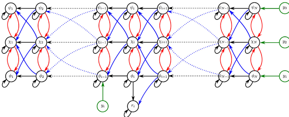
Fig. 4. The graph \mathcal{G}(A^T, C^T) for patterns \mathcal{A} and \mathcal{C} that include matrices A and C , respectively, of system (10), (11), for the case of a three-lane highway stretch where the percentage values of diagonal on-ramp or lateral flows may be nonzero (Model III).
