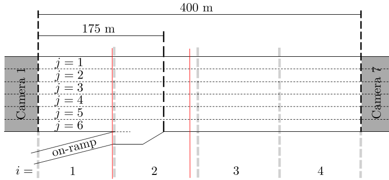
Fig. 6. Graphical representation of the considered stretch of highway I-80 in Emeryville, California, employed in the evaluation of the estimation scheme with NGSIM data.
