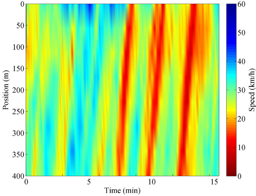
Fig. 8. The aggregated vehicle speeds of lanes j = 2 \dots 6 extracted from the NGSIM data. Congestion shock-waves are spilling back from downstream and cross the entire highway stretch.
