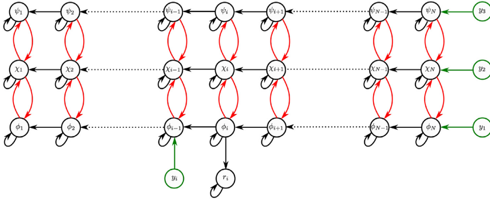
Fig. 3. The graph \mathcal{G}(A^T, C^T) for patterns \mathcal{A} and \mathcal{C} that include matrices A and C , respectively, of system (10), (11), for the case of a three-lane highway stretch with \tilde{p}_{i,j} = p_{i,j} = 0 , for all i and j , when the lateral flows of connected vehicles may be nonzero (Model II).
