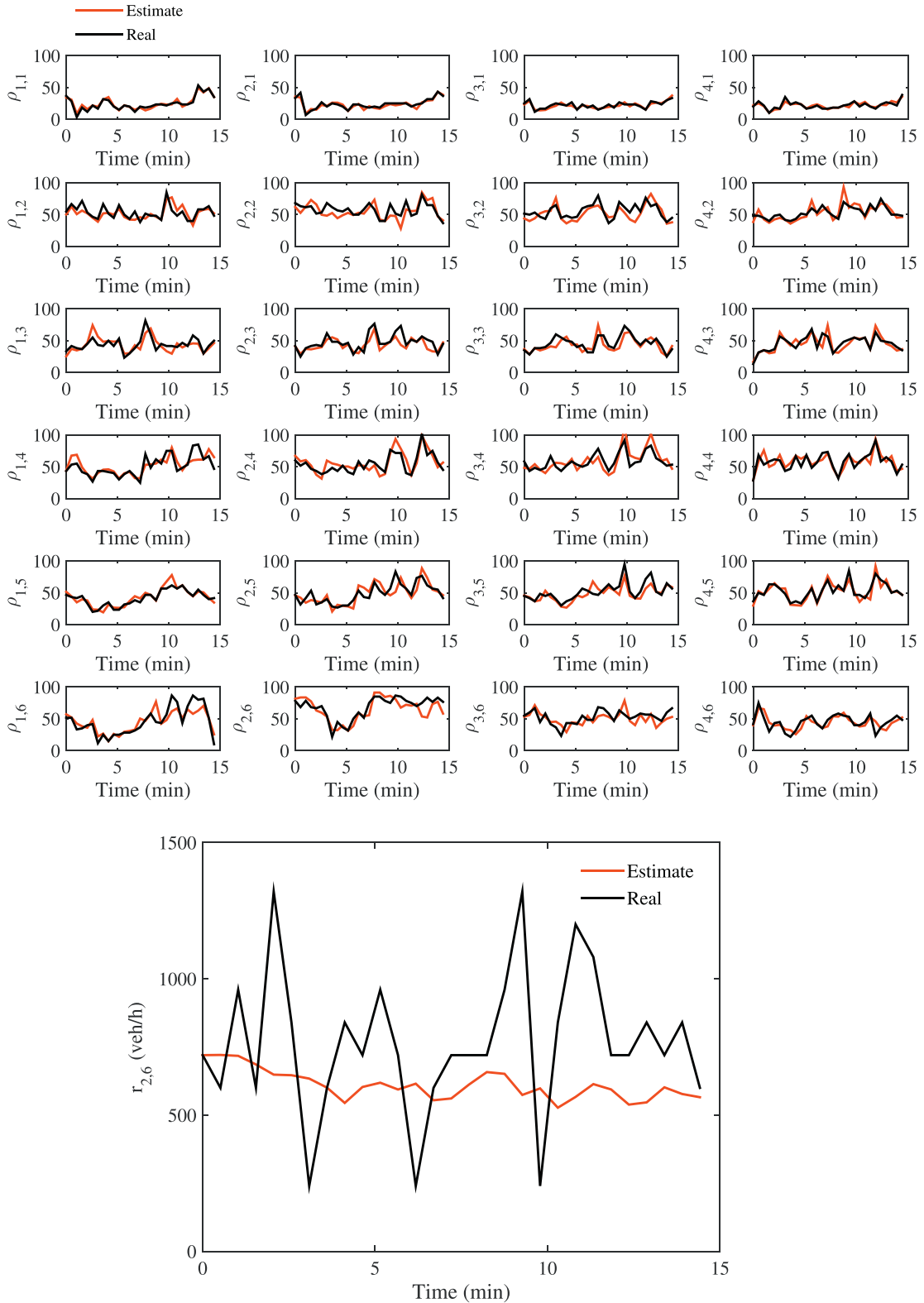
Fig. 9. Top: The estimated densities (red line) produced by the estimation scheme versus the real densities (black line) obtained from the NGSIM data. Bottom: The estimated on-ramp flow (red line) produced by the estimation scheme versus the real on-ramp flow (black line) obtained from the NGSIM data. (For interpretation of the references to colour in this figure legend, the reader is referred to the web version of this article.)
