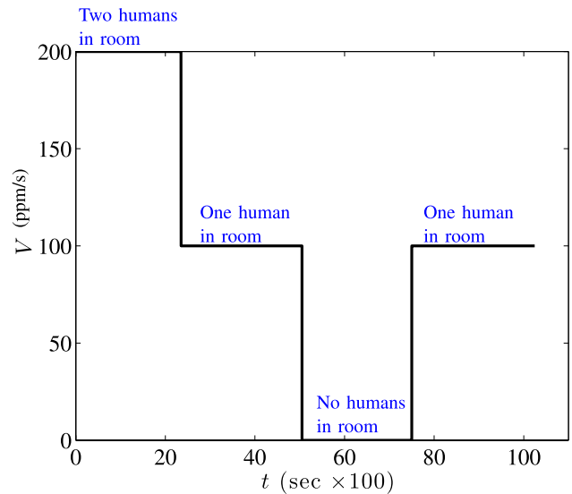
Fig. 13. Input V to the model (1)–(4) emulating the unmeasured \text{CO}_2 generation from the humans for Experiment II.
