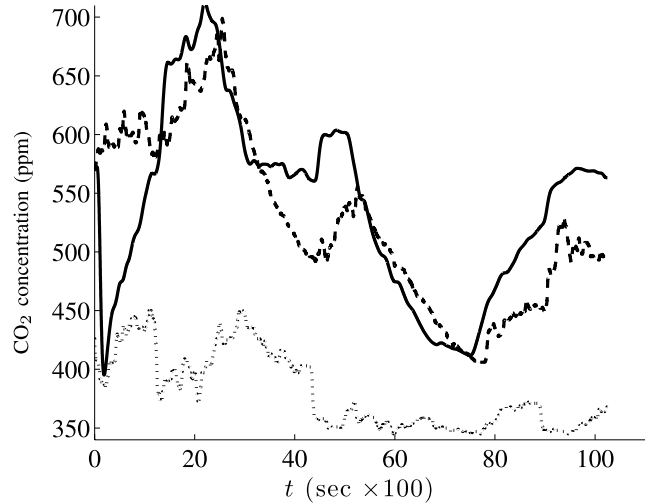
Fig. 12. Solid line—simulated concentration of the \text{CO}_2 at the air return u(1, t) given by the model (1)–(4) for Experiment II. Dashed line—concentration of the \text{CO}_2 at the air return measured by the \text{CO}_2 sensor. Dotted line—input \text{CO}_2 concentration U at the air supply measured by the \text{CO}_2 sensor.
