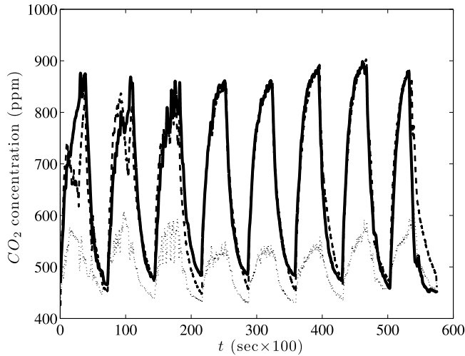
Fig. 10. Solid line—simulated concentration of \text{CO}_2 at the air return u(1, t) given by the model (1)–(4) for Fig. 3 of Experiment I. Dashed line—concentration of the \text{CO}_2 at the air return measured by the \text{CO}_2 sensor, which is shown in Fig. 3. Dotted line—input \text{CO}_2 concentration U at the air supply measured by the \text{CO}_2 sensor, which is shown in Fig. 3.
