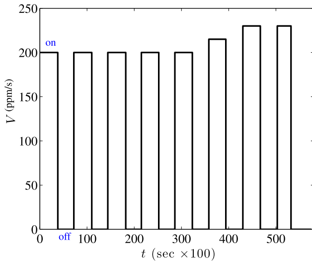
Fig. 11. Input V to the model (1)–(4) from Fig. 3 of Experiment I modeling the concentration of \text{CO}_2 that is released from the pump. When V = 0 , the \text{CO}_2 pump is turned OFF and when V \neq 0 , the \text{CO}_2 pump is turned ON.
