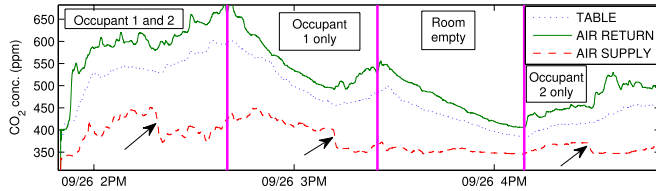
Fig. 7. CO 2 concentrations during Experiment II. Measurements from three locations in the conference room over 3-h experiment are shown. Magenta lines indicate when occupancy changes occurred. The arrows indicate the time instants at which the ventilation rate increases. 3
