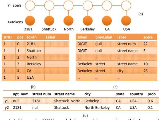
Fig. 1. (a) Example CRF model for an address string; (b) A sample of the TOKEN_TBL table; (c) a sample of the MR table; (d) two possible segmentations Y_1, Y_2 .
