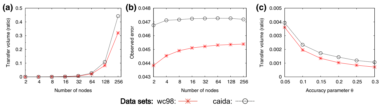
Fig. 8 Subfigures a and b present the network cost and observed error for different network sizes, whereas subfigure c presents the effect of the value of \theta on the network cost
