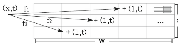
Fig. 1 Adding an element to the ECM-sketch
