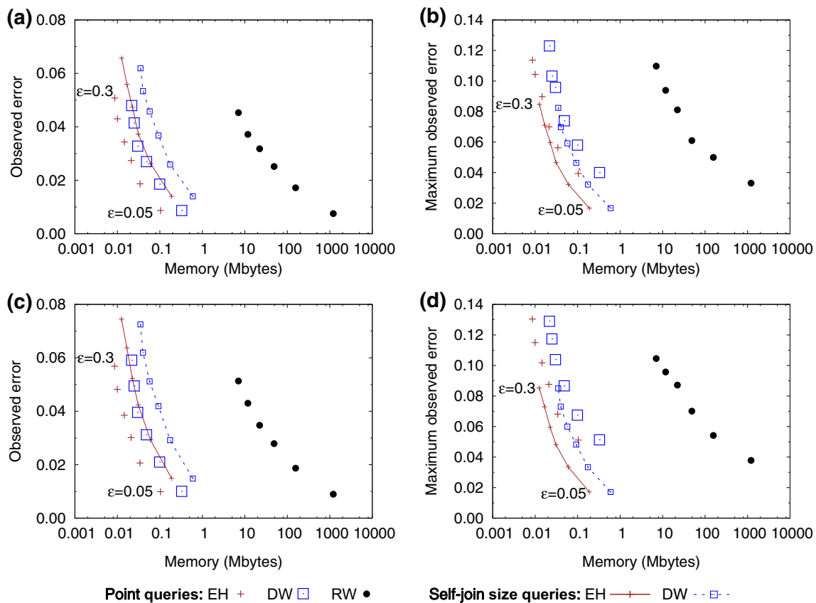
Fig. 5 Average and maximum observed error in correlation to memory requirements for a centralized setup. Subfigures a and b present the results for the wc98 data set, and subfigures c and d for the caida data set. The points correspond to \epsilon \in \{0.05, 0.1, 0.15, 0.2, 0.25, 0.3\}
